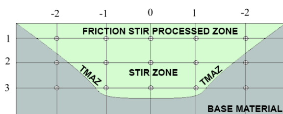
Fig. 2. Microhardness
