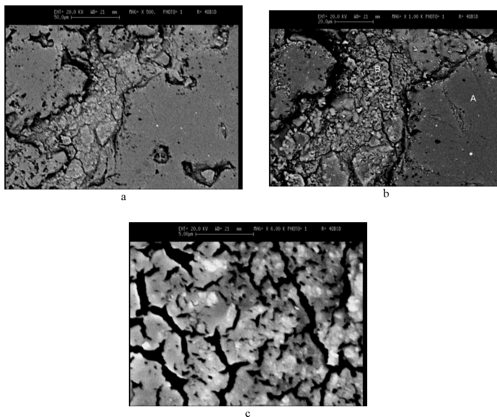
Fig. 10. SEM micrographs of MC sample after firing at 1400^{\circ}C , in magnification of a) \times 500 , b) \times 1000 c) \times 6000
