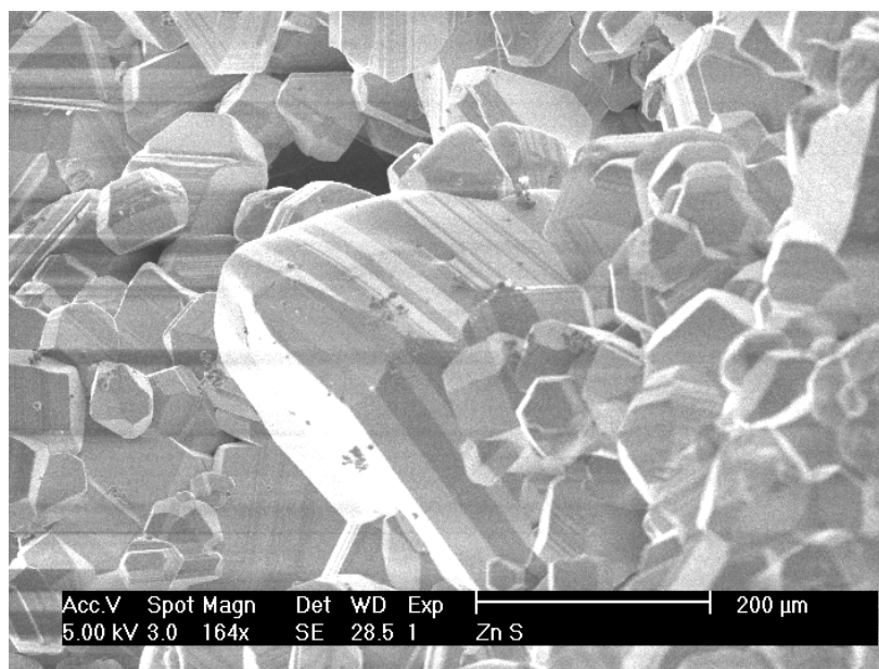
Fig.3. ZnS Crystallites grown at 1050 oC with \Delta T=50 oC.
