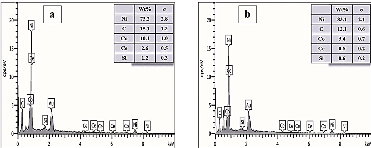
Fig. 4. EDS results of the coatings obtained at a frequency of 10 Hz, duty cycle of 10%, and different current densities: a) 0.1, and b) 0.3 A/cm²
