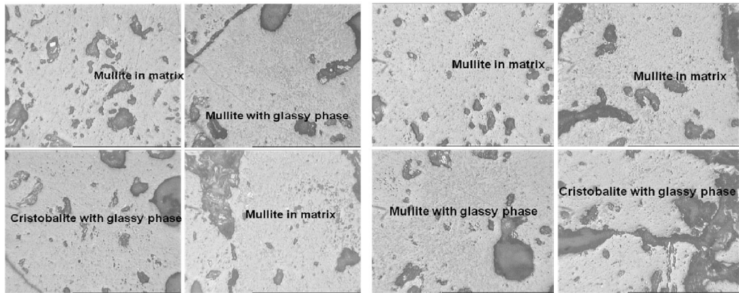
Fig. 9 (c) Microscopic studies of the bricks made from overflow samples
